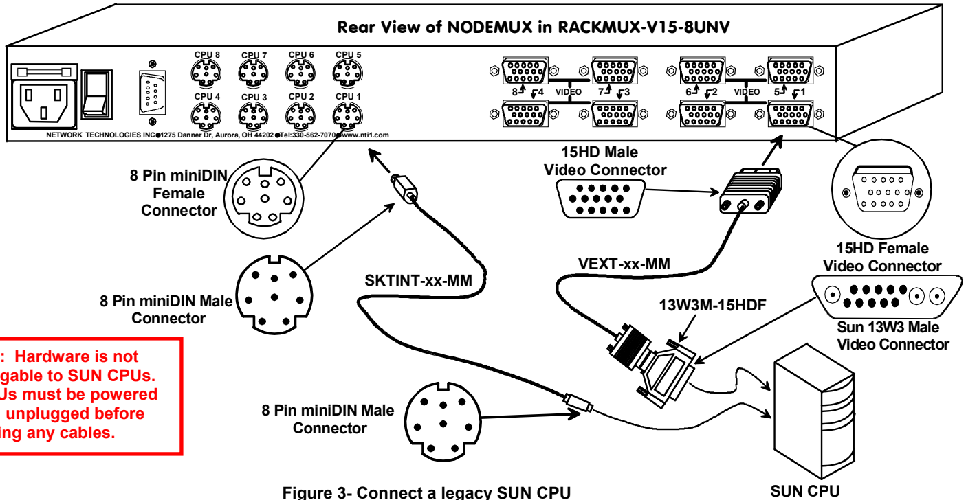
Figure 3- Connect a legacy SUN CPU
